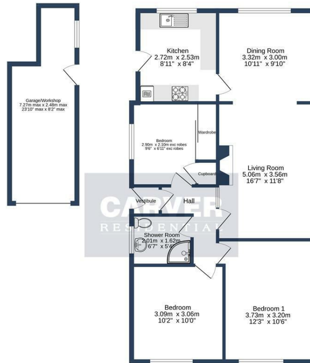
GROUND FLOOR 101.1 sq.m. (1088 sq.ft.) approx.
